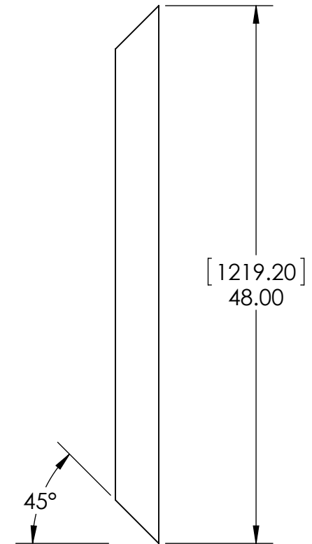
4x4 Cedar Support 4
