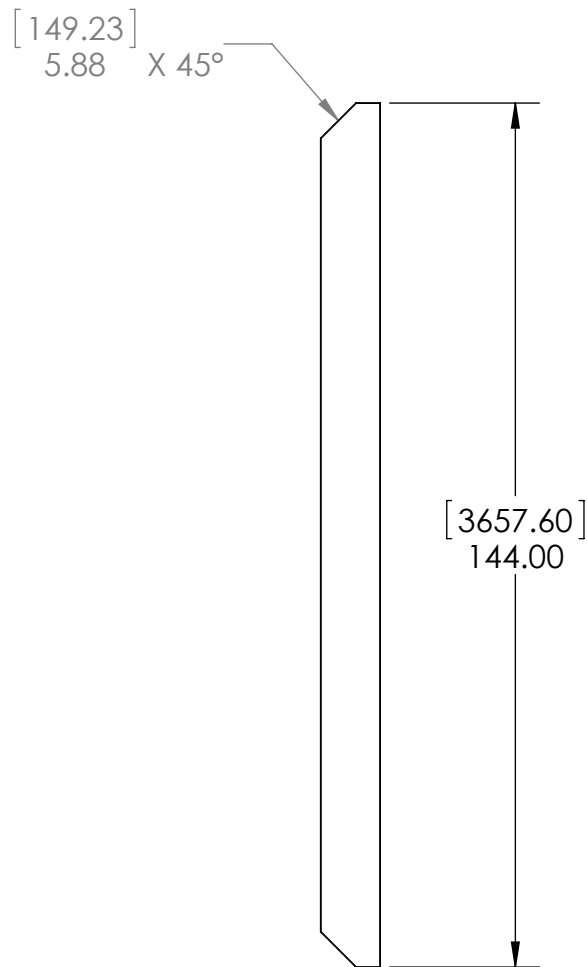
4x10 Cedar Board 12 with chamfered cuts
