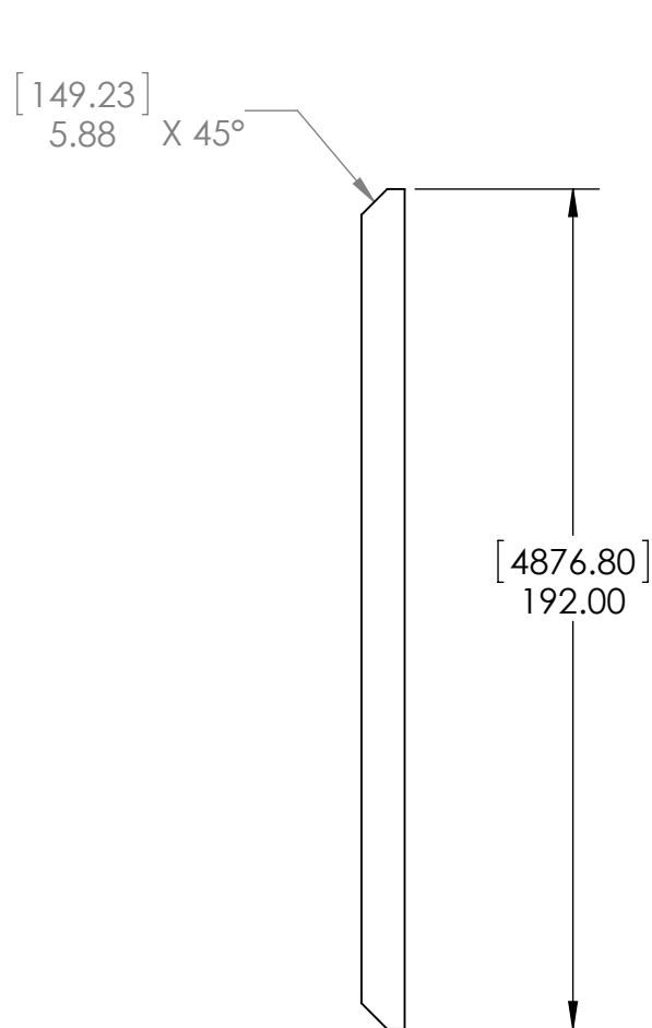
4x10 Cedar Board 16 with 45 cuts
