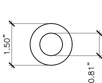
WASHER X2
