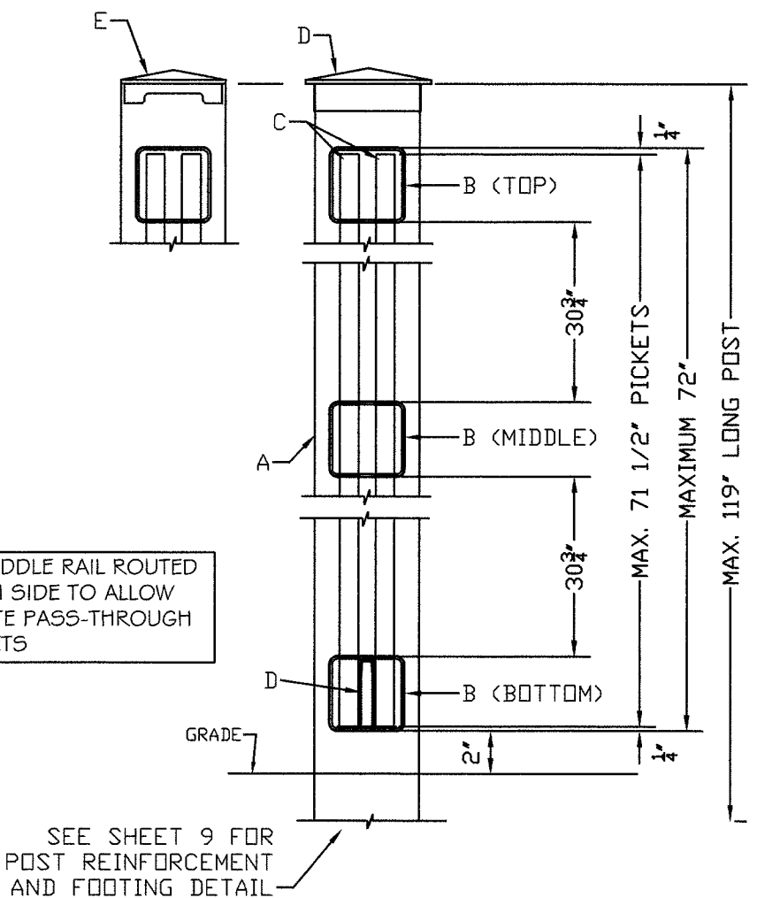
VERTICAL SECTION
