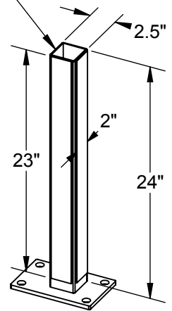
Gate Shoe
