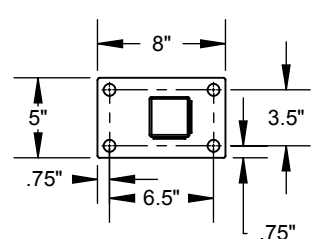
Gate Shoe
