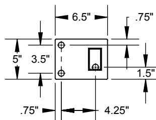
End Shoe
