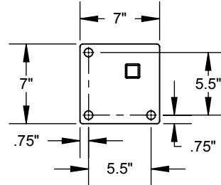
Corner Shoe
