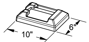
Gate Shoe Skirt
