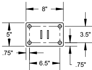
Line Shoe
