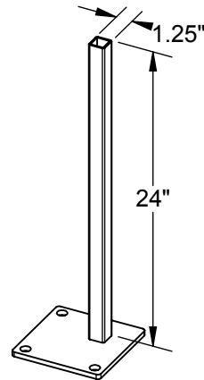
Corner Shoe
