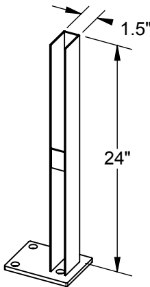
End Shoe
