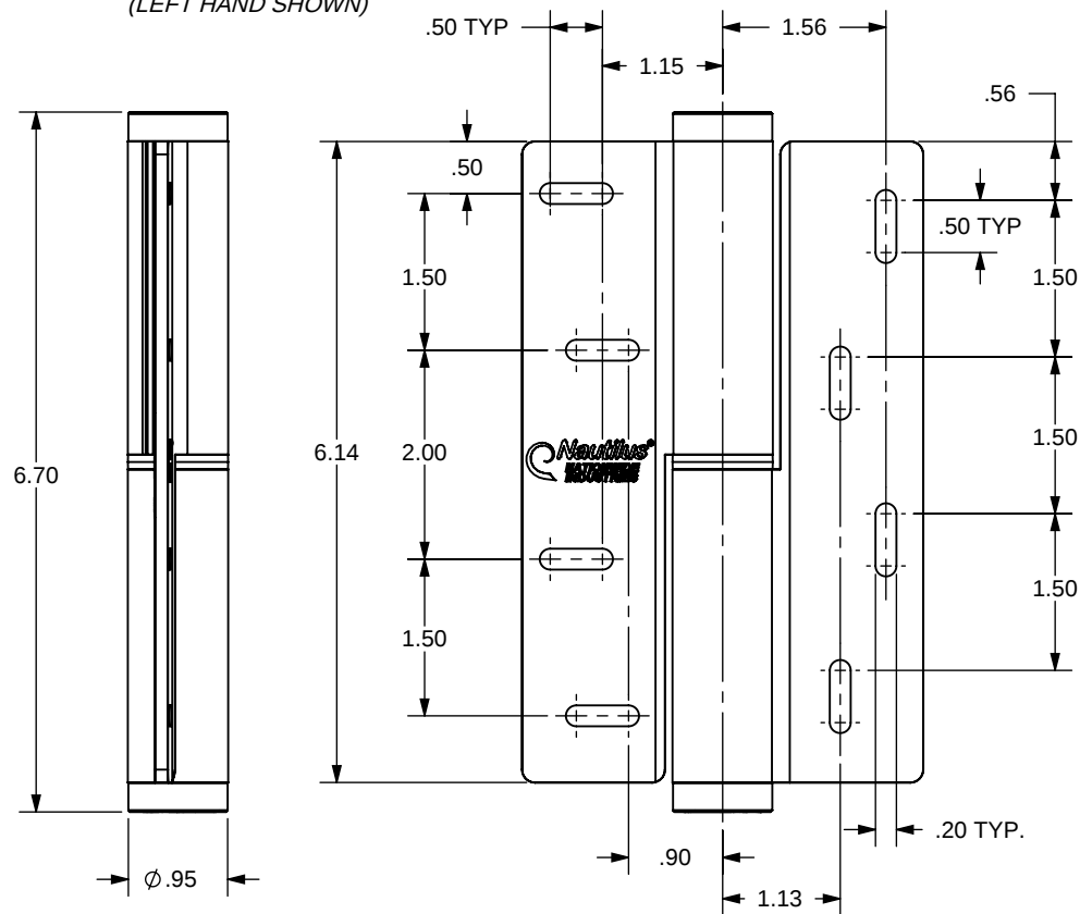
HINGE ASSEMBLY (LEFT HAND SHOWN)
