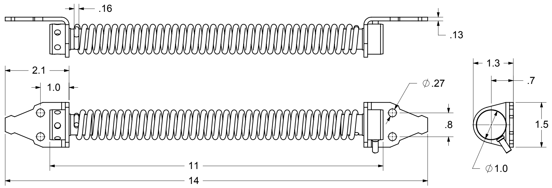
SPRING ASSEMBLY
