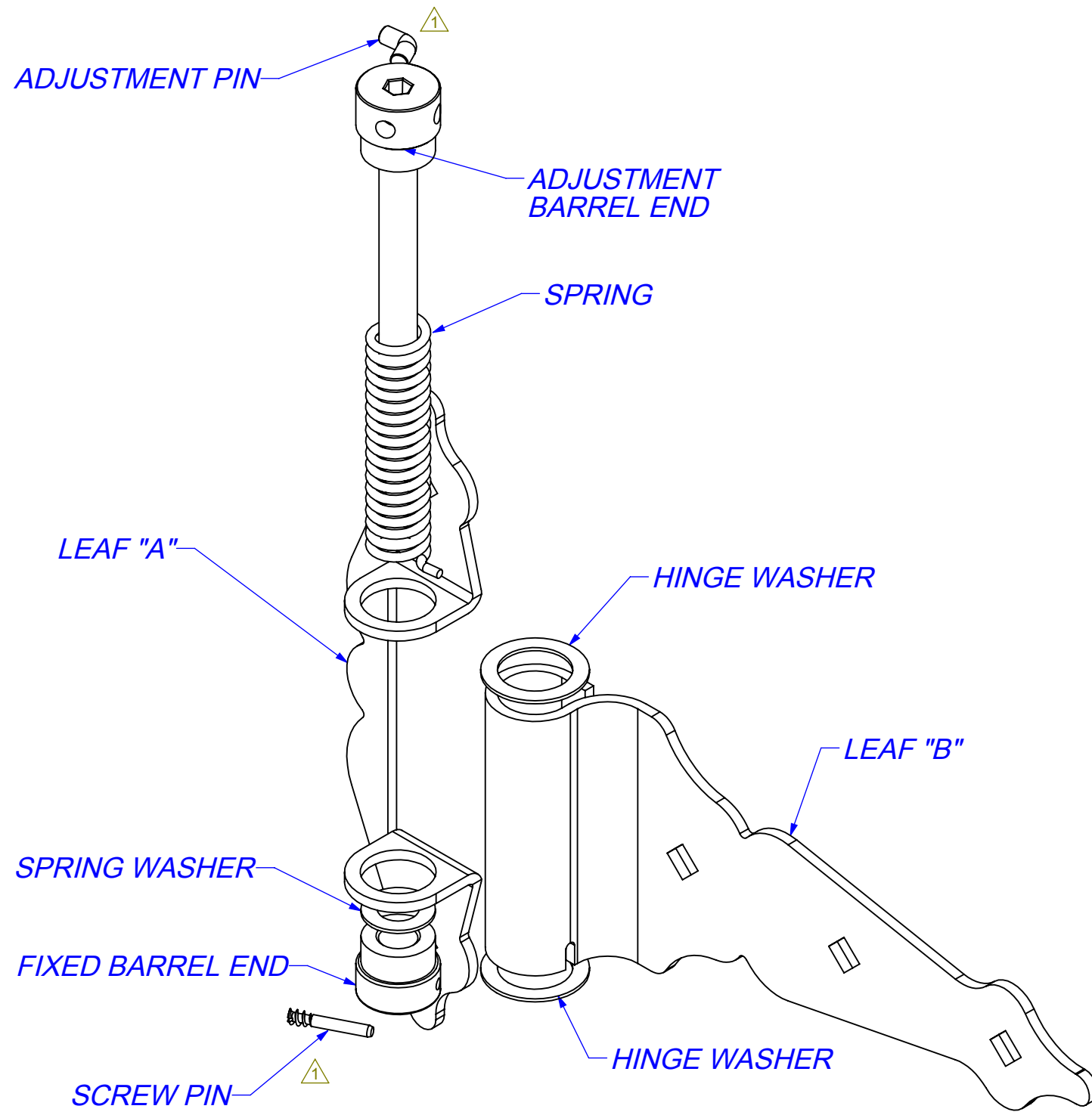
HINGE ASSEMBLY (EXPLODED VIEW)
