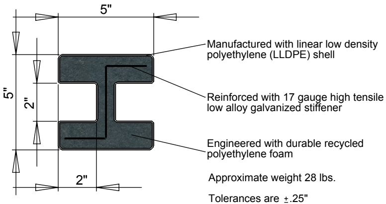
Line post cutaway
