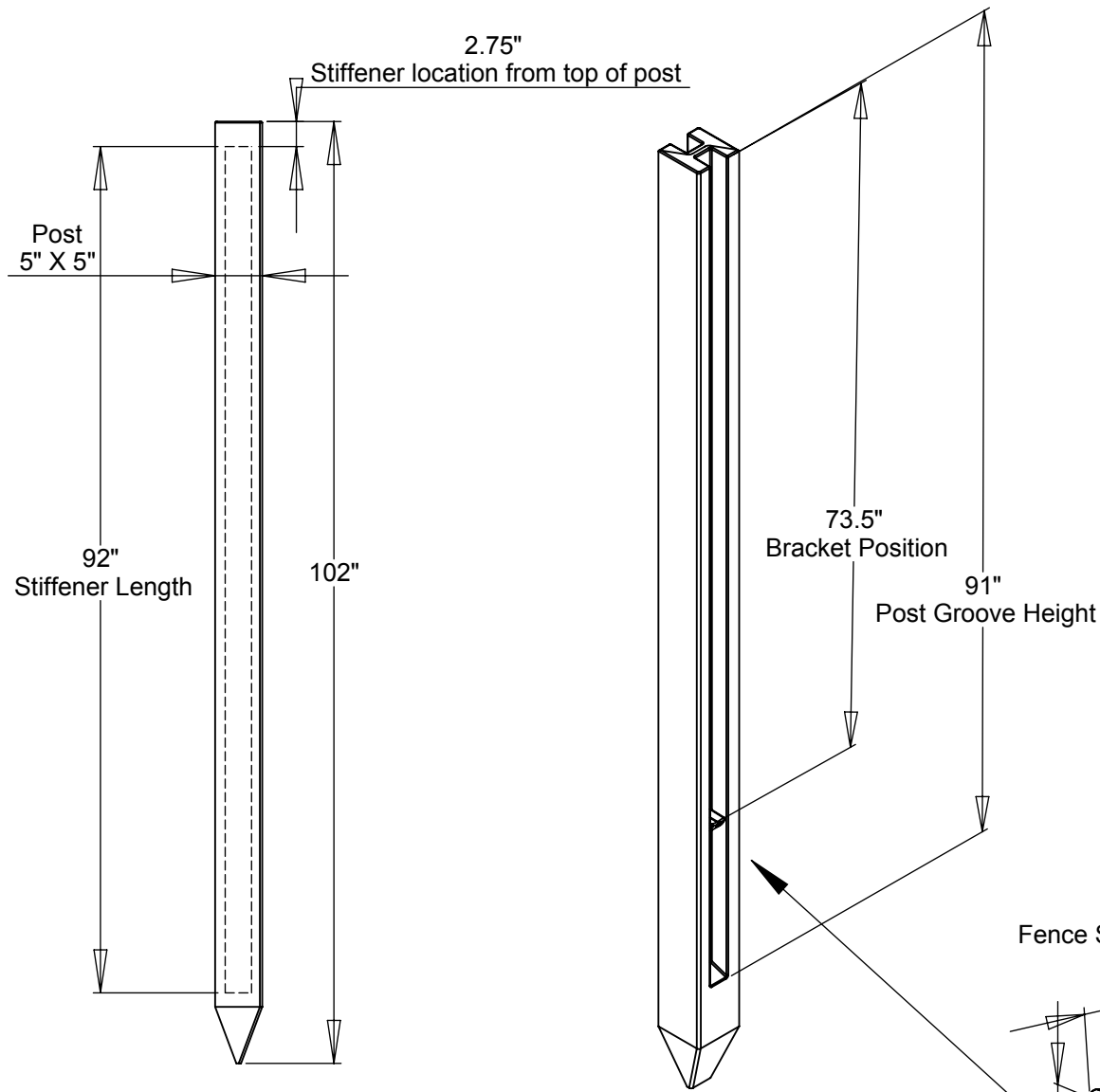
Line post cutaway
