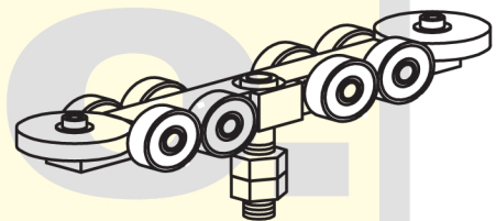
Truck Assembly With sealed roller bearings
