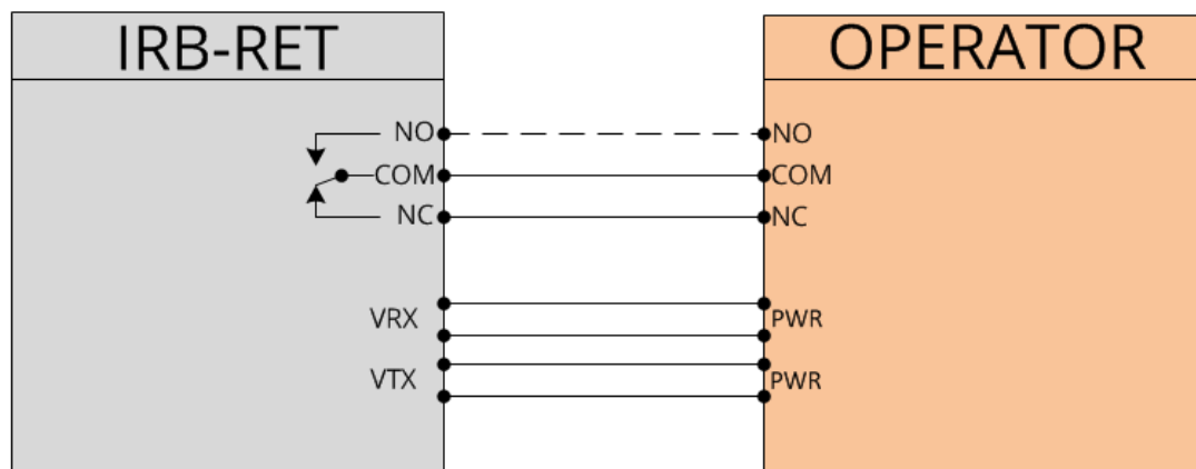
WIRING DIAGRAM C
