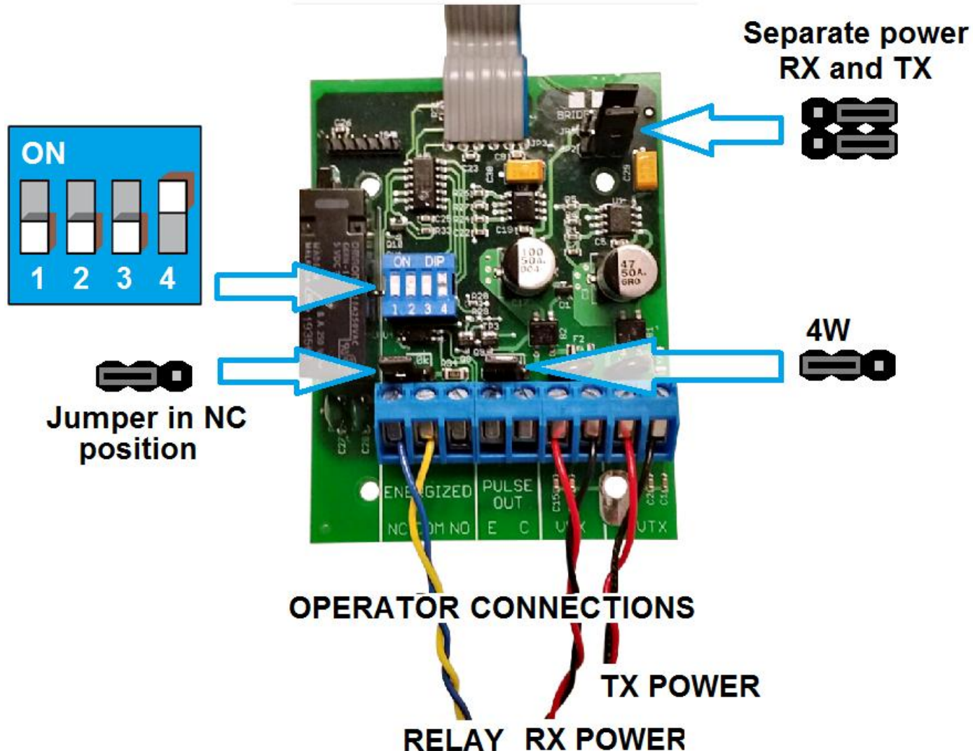
WIRING DIAGRAM C
