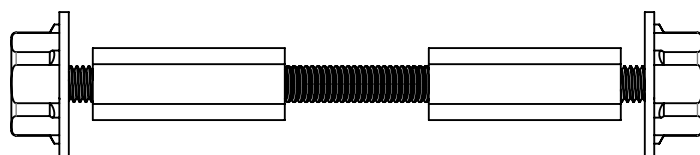
Assembly, OWT Timber Bolt 6-8" 56650-10
