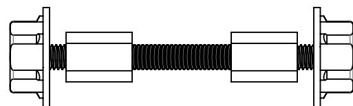
Assembly, OWT Timber Bolt 4-6" 56649-10
