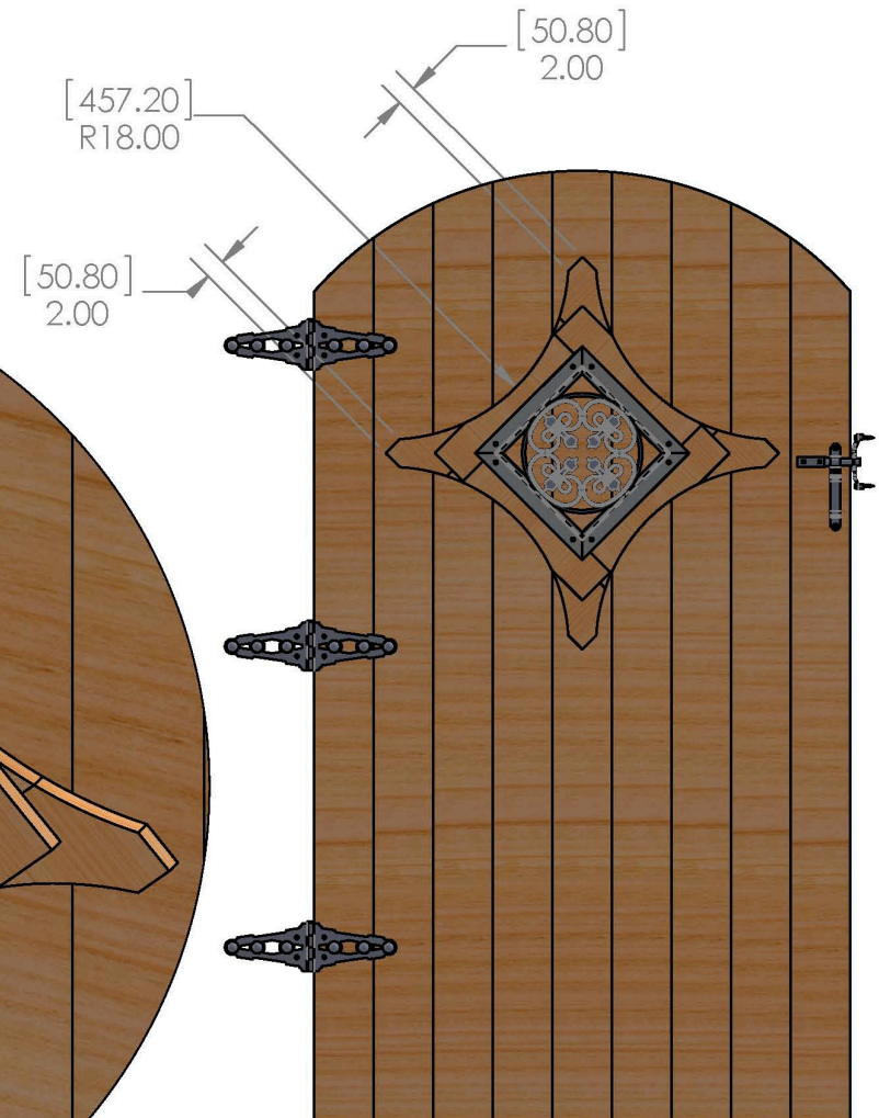
2 layer Shadow box with radius cut
