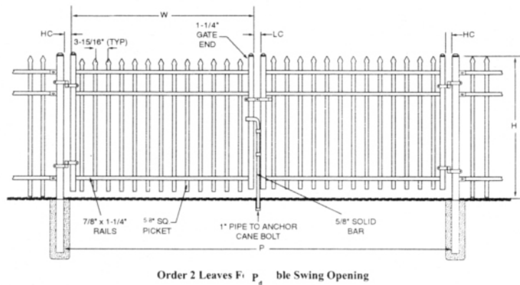
Order 2 Leaves For P_d Double Swing Opening
