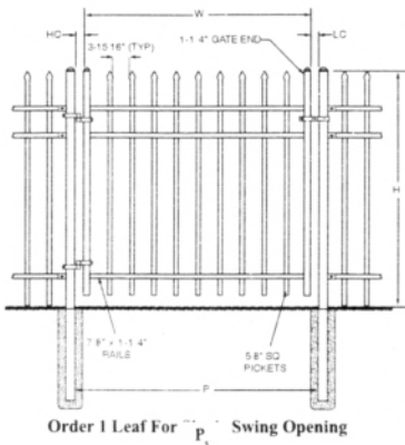
Order 1 Leaf For P_s Swing Opening
